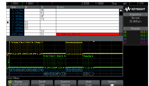
2000 X-Series' hardware-based serial decode provides the industry's fastest update rate while decoding serial buses
