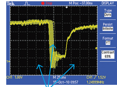
TDS2000C after 40 seconds—it never sees the glitches and shows limited signal jitter due to its slow update rate of 180 wfms/s
